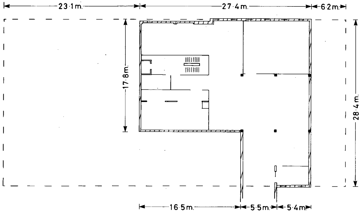
FIGURE 1: BASEMENT PLAN
