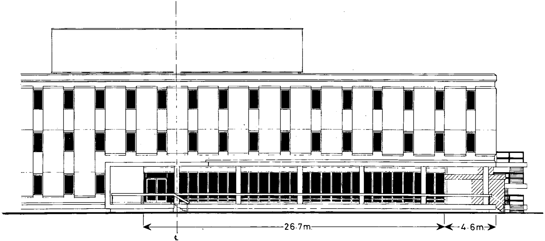
FIGURE 7: EAST ELEVATION (NORTH END)
