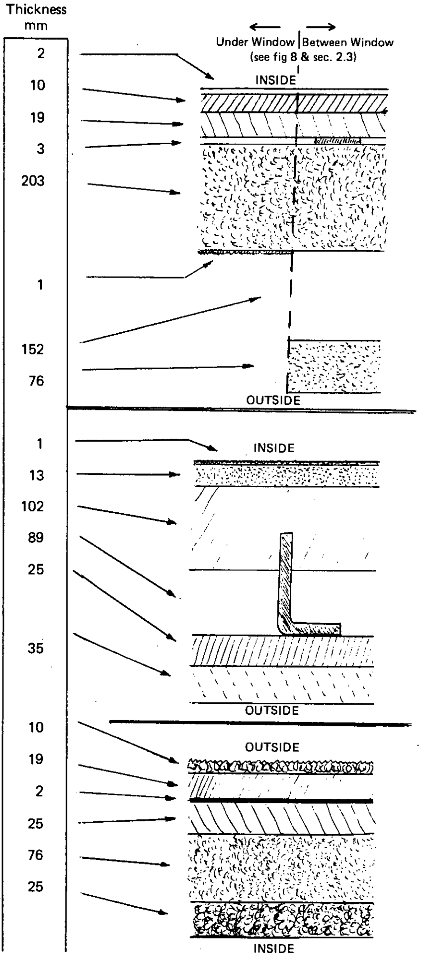
FIGURE 11: FABRIC CONSTRUCTION
