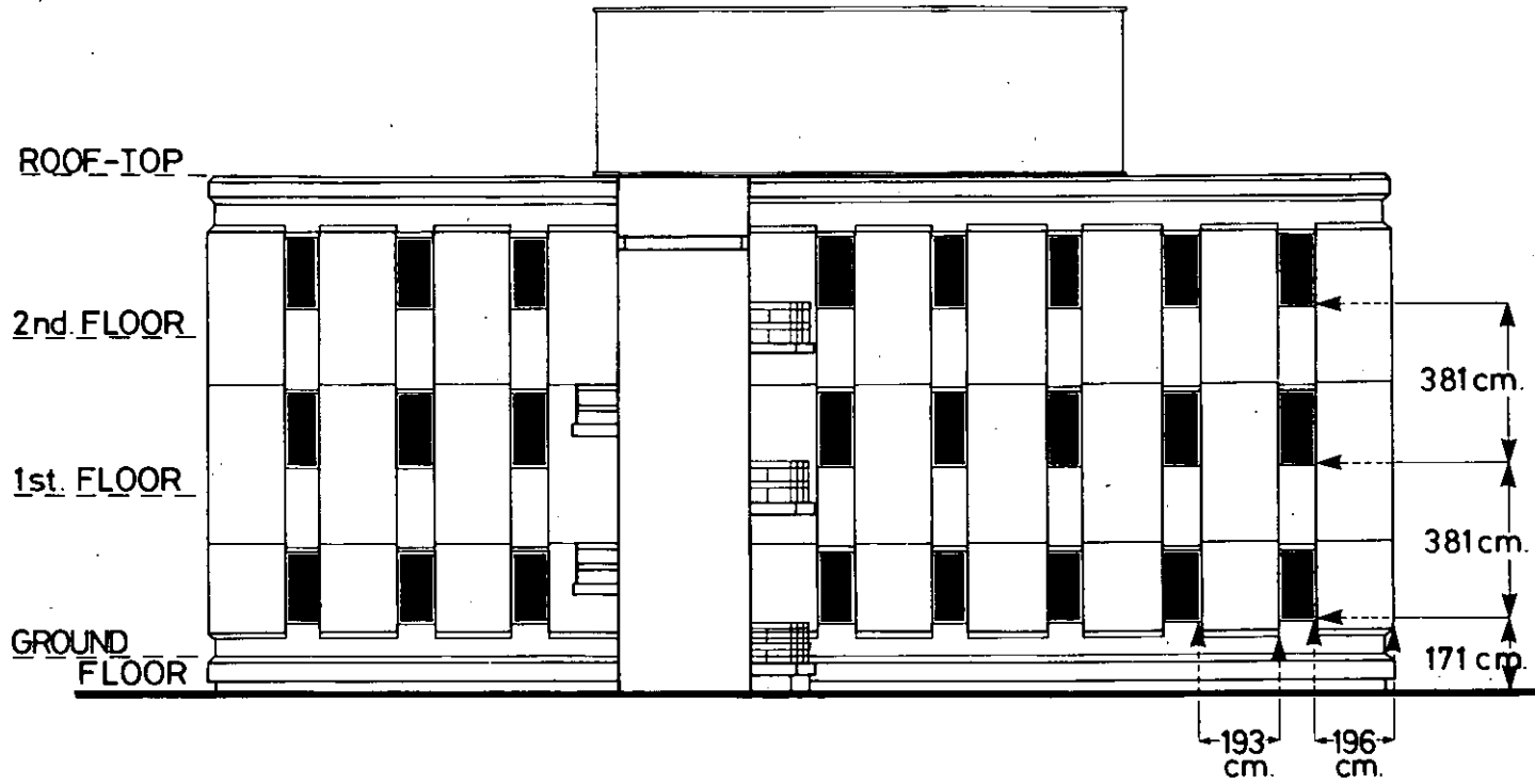
FIGURE 6: SOUTH ELEVATION
