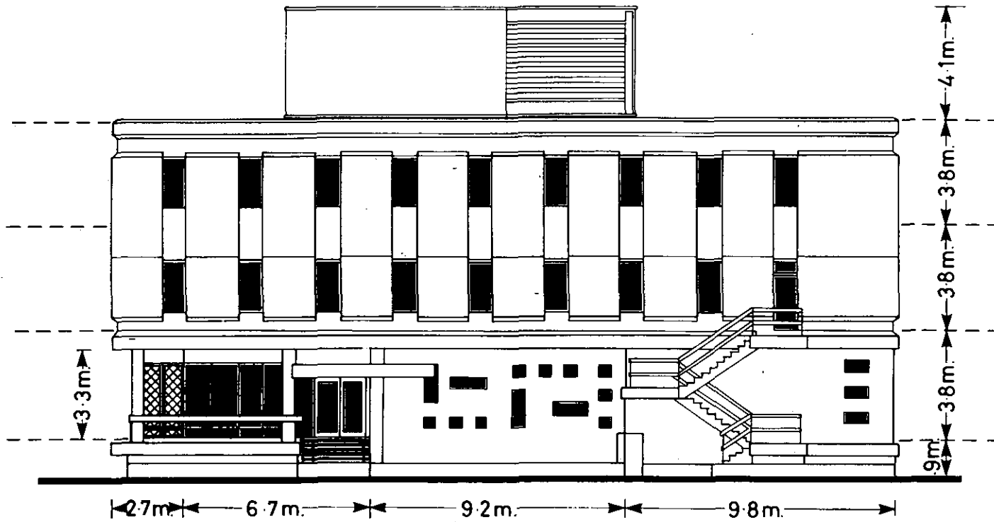
FIGURE 5: NORTH ELEVATION
