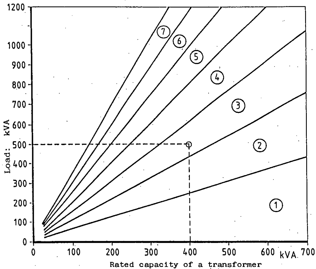
Figure 3.3.B. - Optimum number of transformer units of equal nominal power operated in parallel depending on the load.
