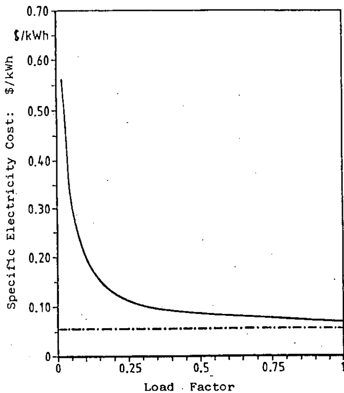
Figure 2.1.A. - Specific electricity costs as a function of the load factor
