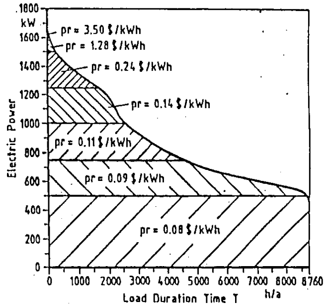
Figure 2.1.C - Typical daily load cycle and yearly duration curve of the load of a large German hospital
