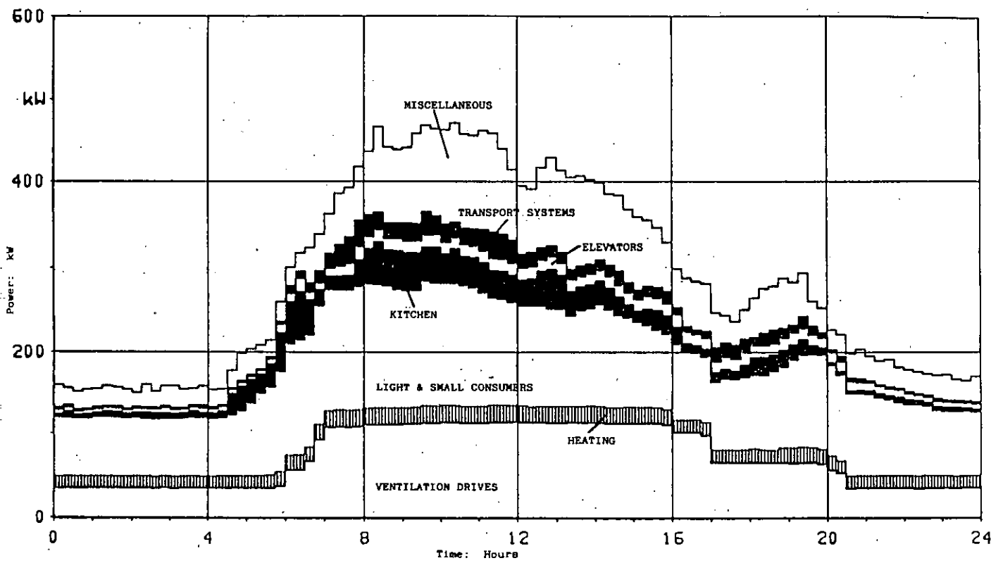
Fig. 2.2.A. - Average load cycle of the electricity consumption of Hospitals with 434 beds
