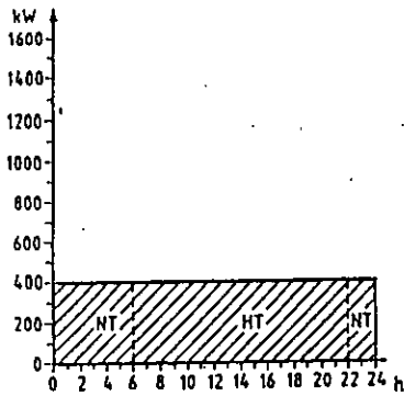
Figure 2.1.D. - Two extremes of load cycles with equal energy consumption
