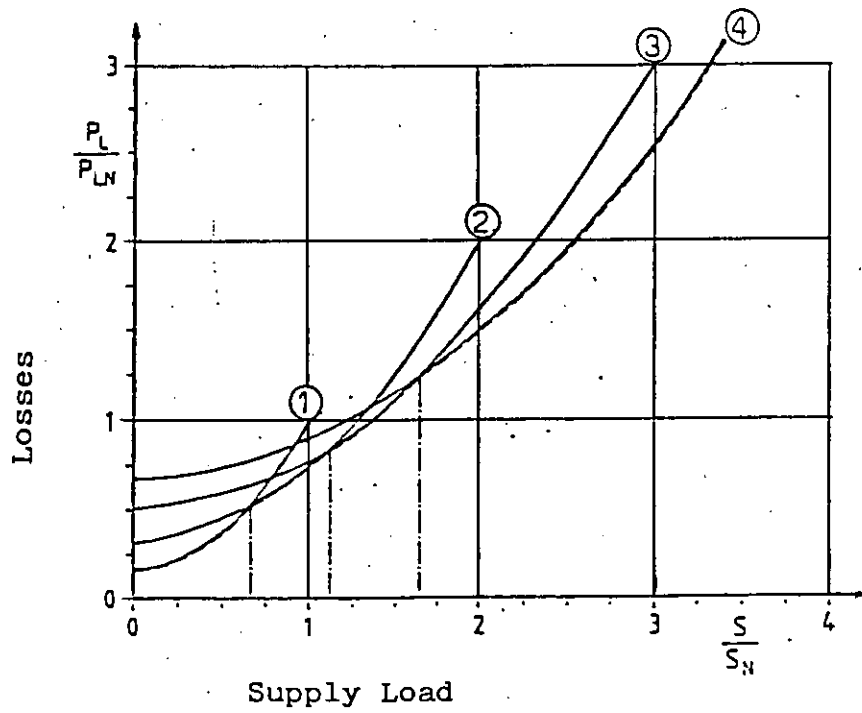
Figure 3.3.A. - Losses of one or more transformers operated in parallel depending on the load
