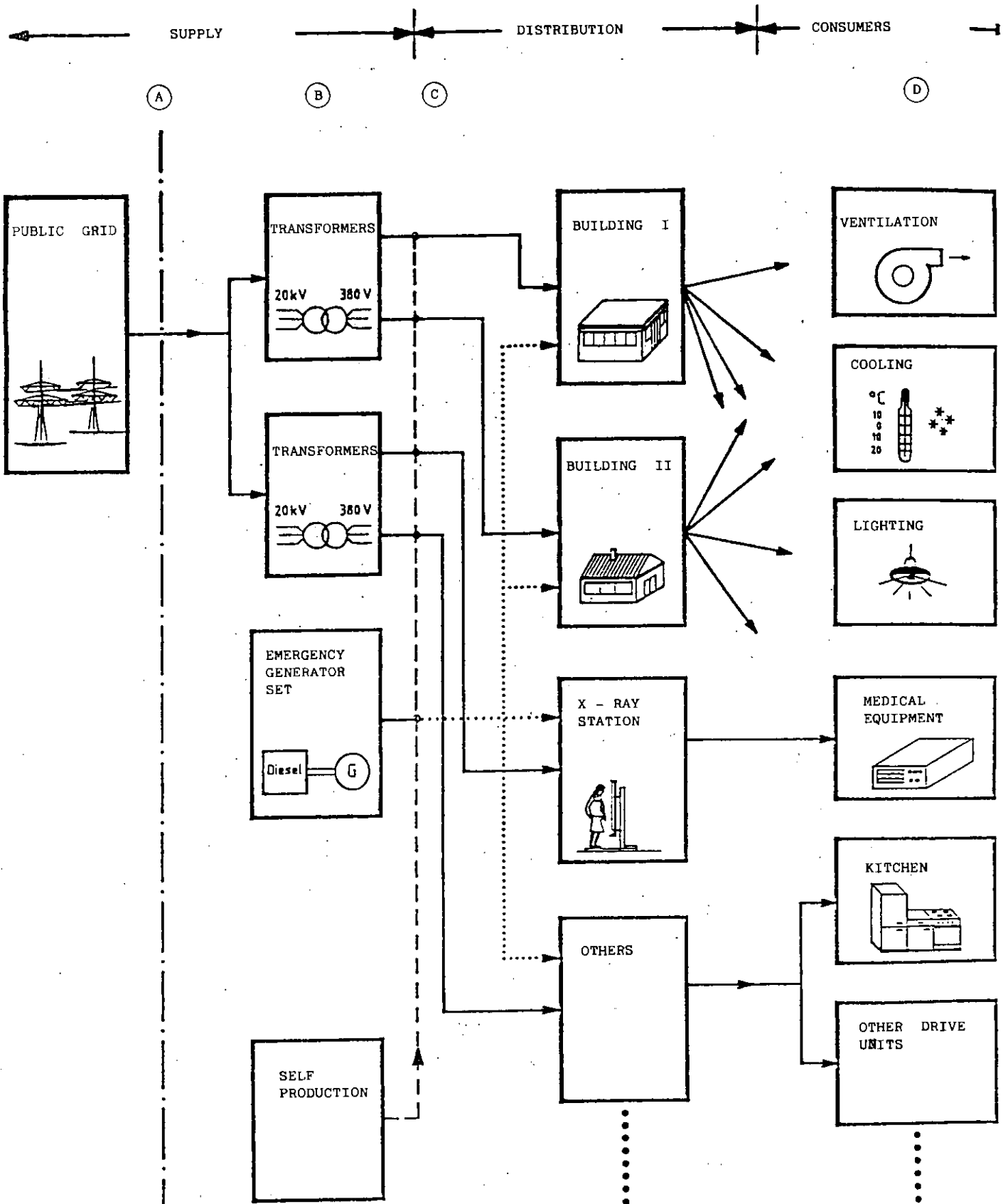
Fig. 1.A. - Block diagram of the electrical system with:
