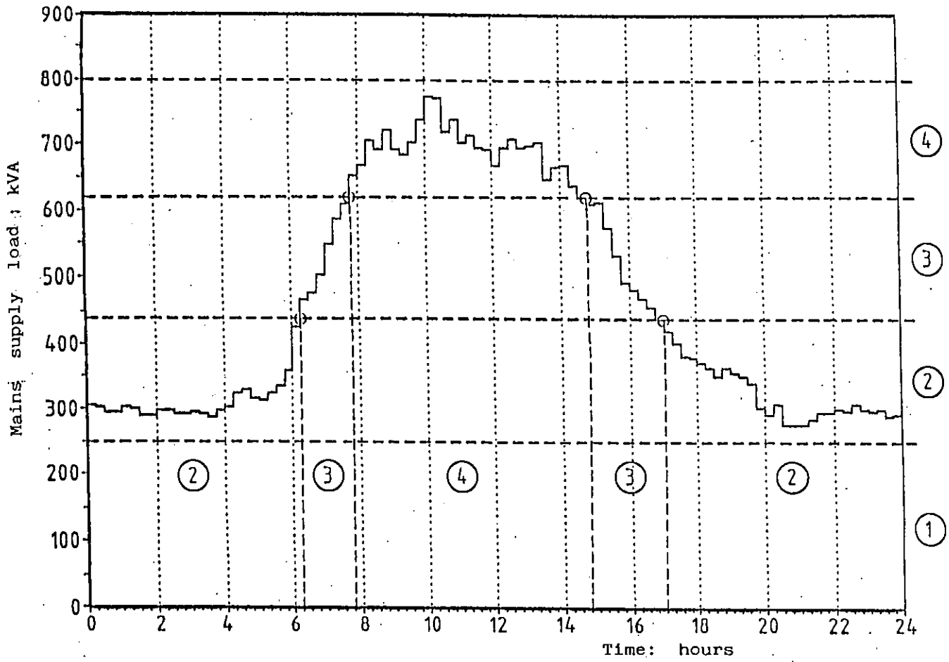
Figure 3.3.C. - Example of a transformer schedule
