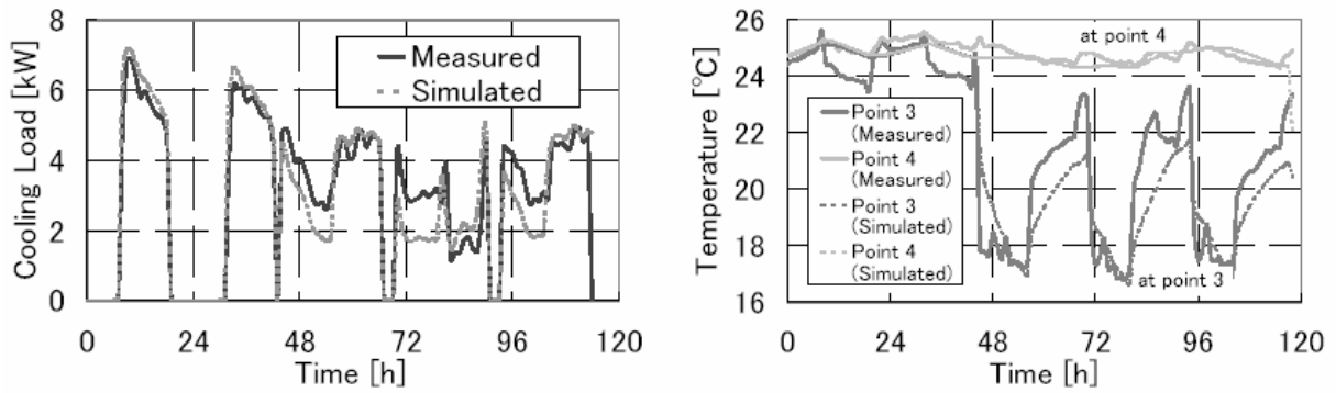
Figure 3.37 – Comparison of measured and simulated results (left: cooling load, right: lower surface temperatures of slab at points 3 and 4)
