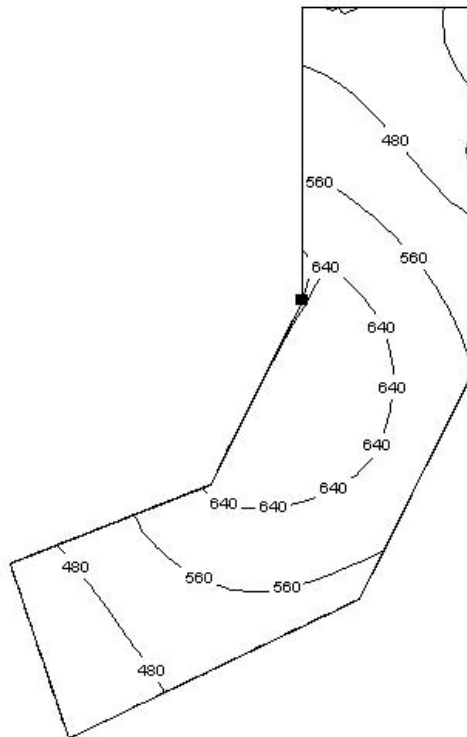
Figure 10-20. Illuminance distribution on working plane (only artificial light).
