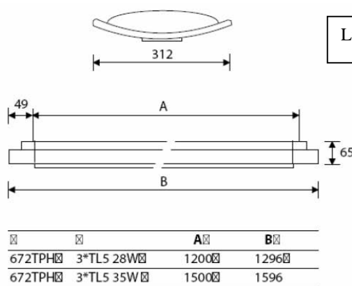
a) Photometry of the luminaire b) Geometry of the luminaire
