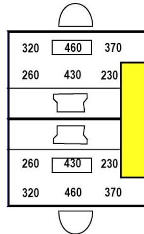
Figure 10-26. Direct-indirect suspended luminaire.
