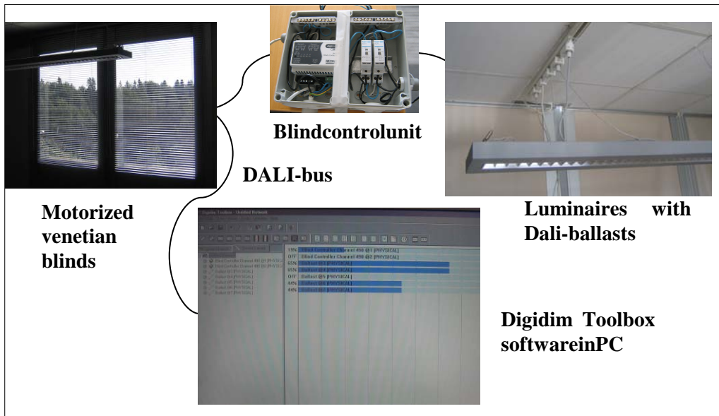
Figure6-49. TheintegratedcontrolsysteminterfacedtoDALI bus.
