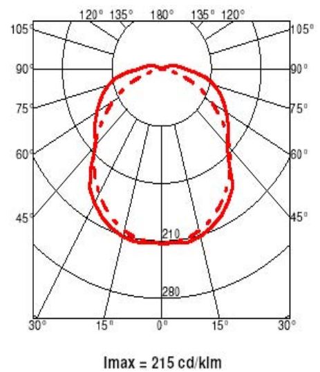
Figure10 -47. Luminairecharacteristics: Intensitydiagram.
