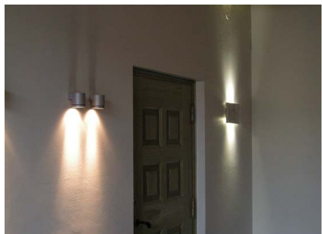
Figure10 -36. 2x35Wtungstenhalogenlampsreplaced by2x3WRebelLEDsgivinglightupanddown.
