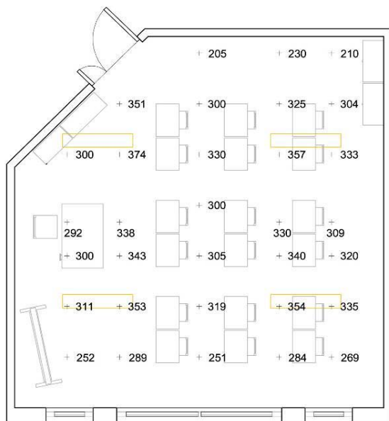
Figure 10 -80. Illuminances on the workplane due to daylight: measured on 21th December at 12 am under overcast sky conditions (external illuminance 5000 \text{ lx} ).
