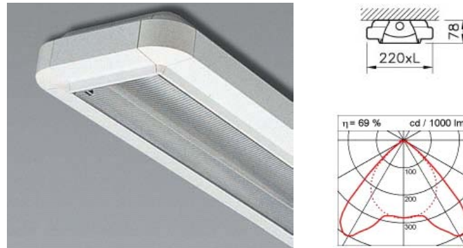
Figure 10-3. Characteristics of the luminaire.
