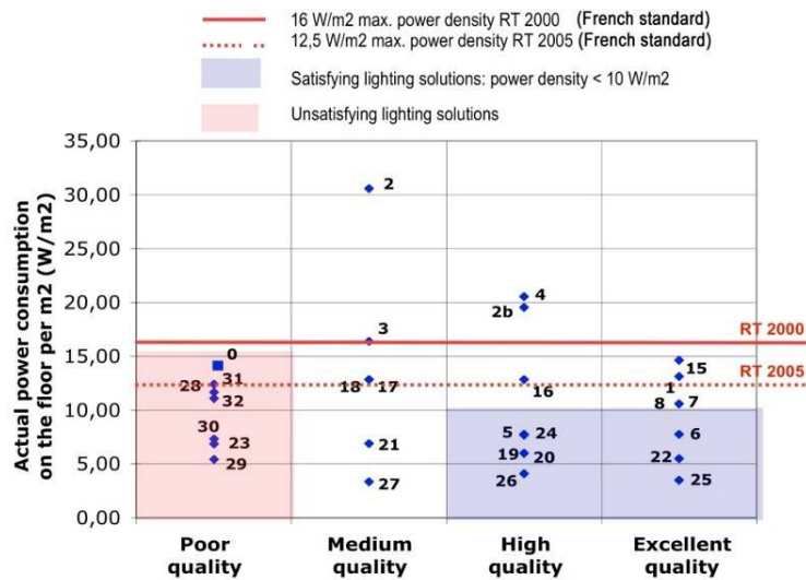
Figure 10-24. Perceived visual quality as a function of the electric power density for lighting for 26 lighting schemes.
