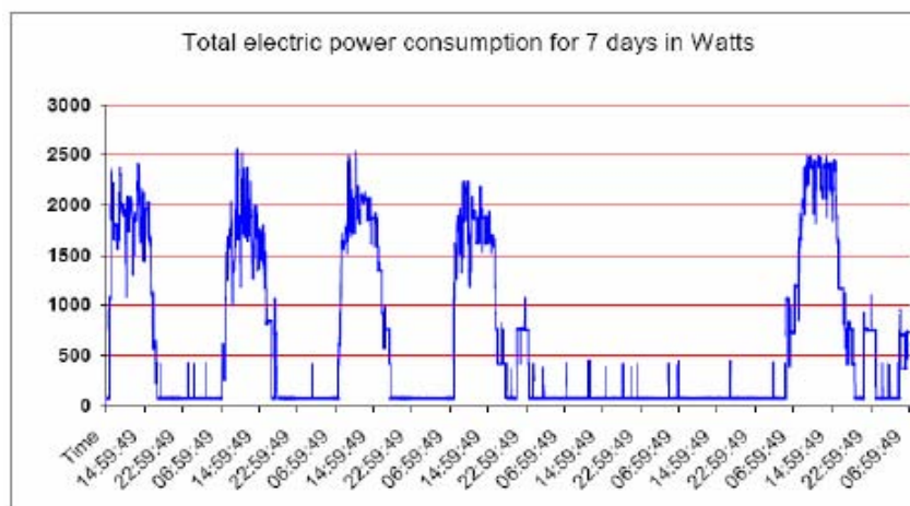
Figure 10-11. Profile of the total power consumption of the local area during 7 days.
