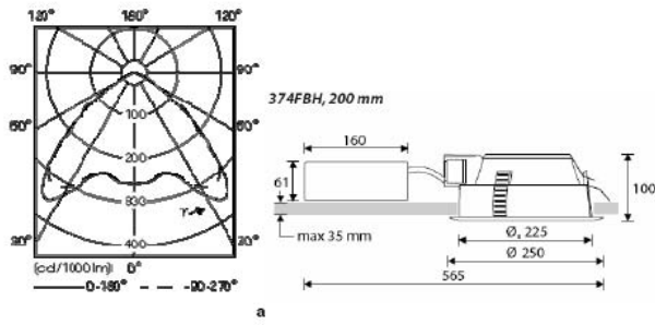
a) Photometry of the luminaire b) Geometry of the luminaire
