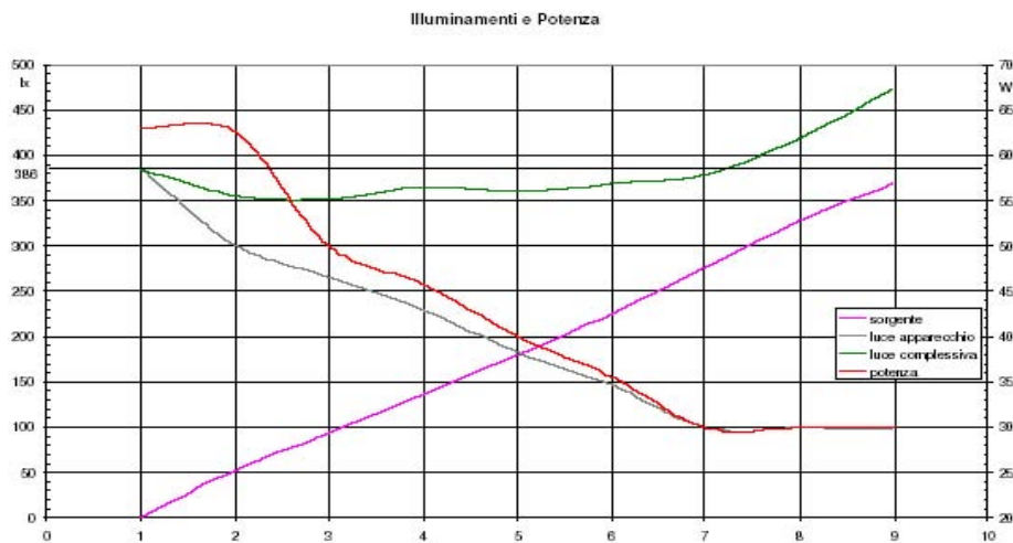
Figure10 -49. Exampleofdimming:dependingonanexternallight contribution (simulating daylight), power and illuminance from the luminaire are shown. Totalilluminance(externalsourceandluminaire)isalsoshown.
