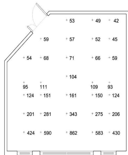
Figure 10 -81. Illuminance values on the workplane at full power (artificial light).
