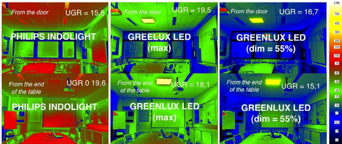
Figure 10-41. Luminance distribution of the measured room
