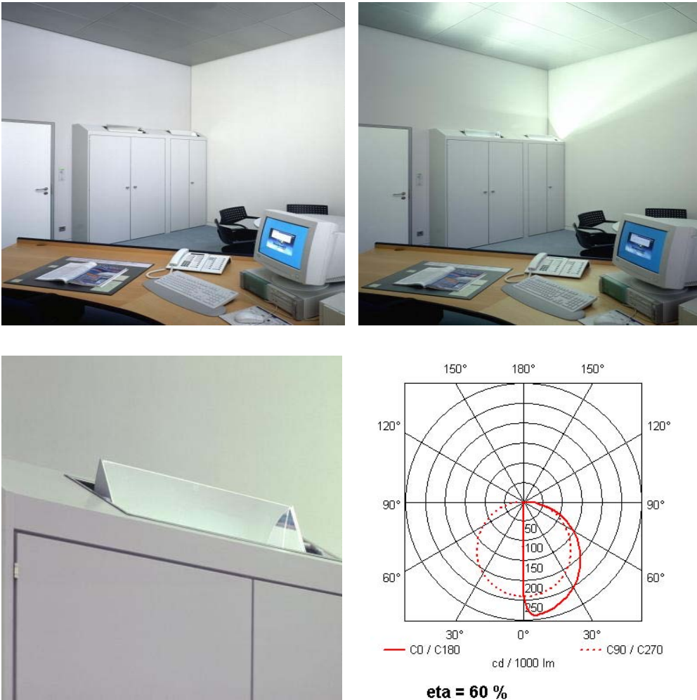
Figure 10-16. Luminaires installation .
