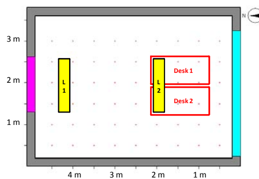
Figure 10-2. Office plan with luminaires position.
