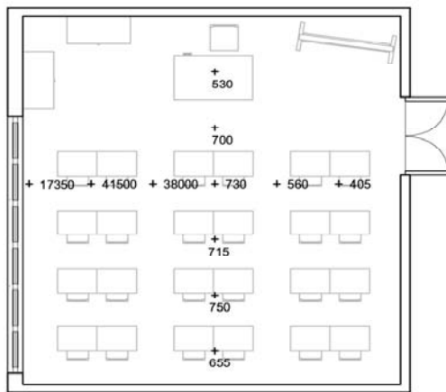
Figure10 -86. Illuminance on the work plane due to daylight: measured on 18th November at 12 am under sunny sky conditions(external illuminance 48000lx).
