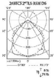
Photometry of the luminaire
