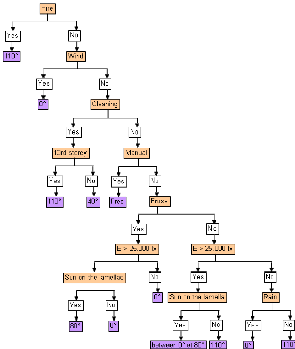
Figure6-45. Structureofthecontrolstrategyofthedaylightin
