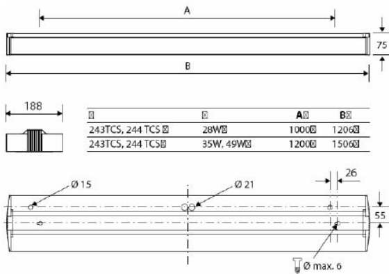
Geometry of the luminaire
