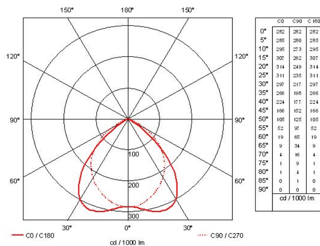
Figure 10-84. Photometry of the luminaire.
