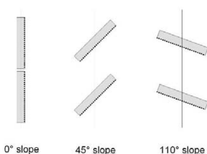
Figure 6-42. Different louver positions.
