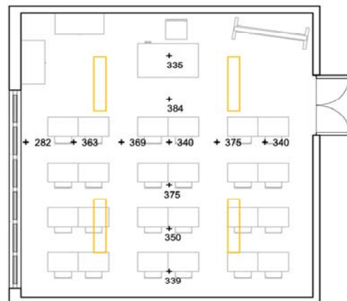
Figure 10 -87. Illuminance values on the work plane at full power (artificial light).
