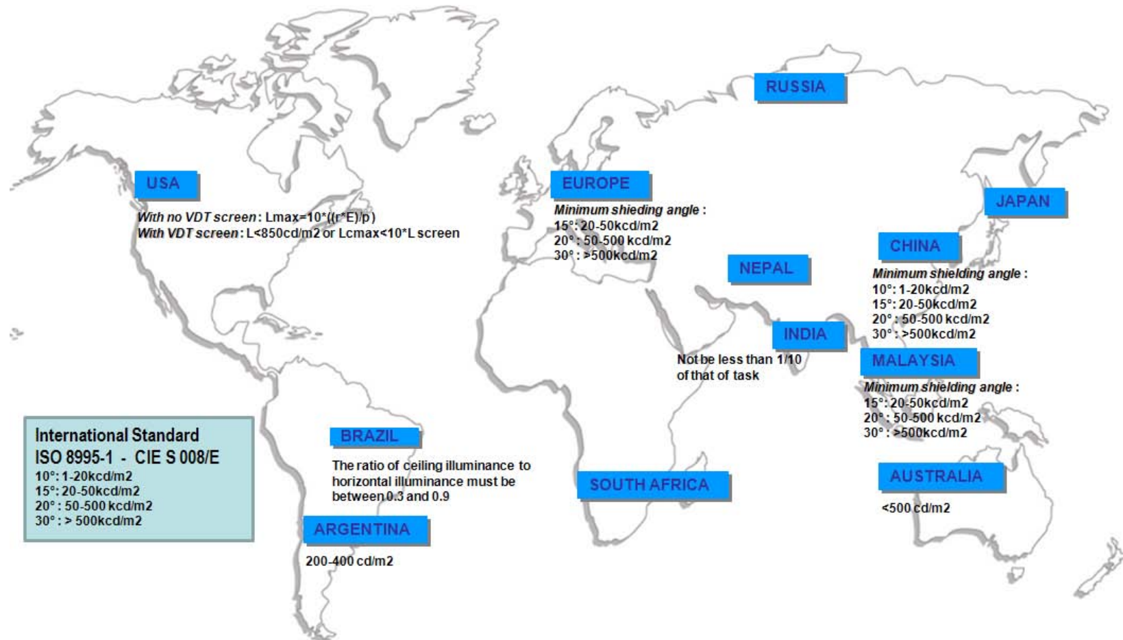
Figure 4-6. Ceiling luminance and shielding angle.
