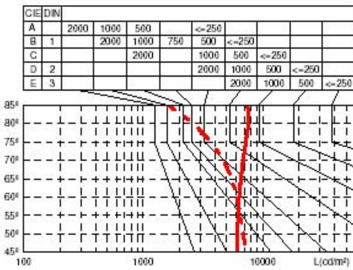
Figure 10 -46. Luminaire photometric characteristics (luminances(cd/m 2 )vsangles).
