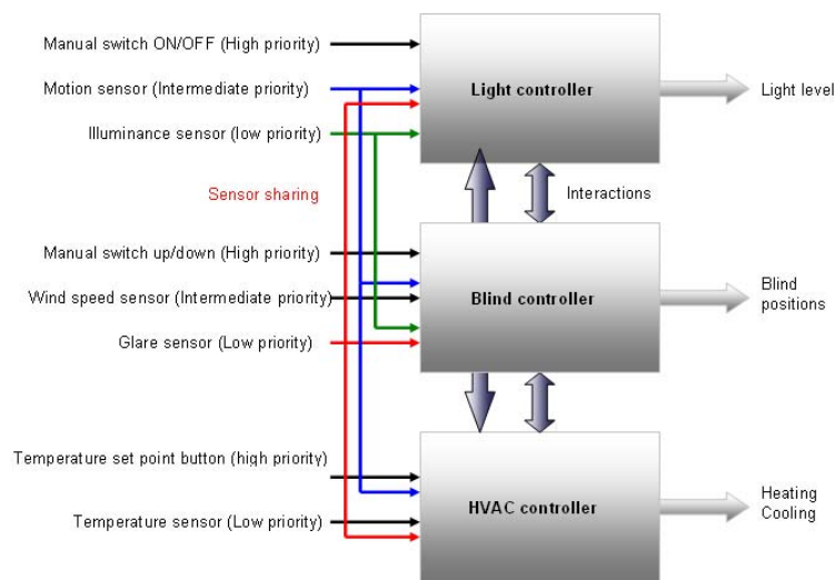
Figure6-13. Interactionofthesensorsonthedifferentcontrol levels.
