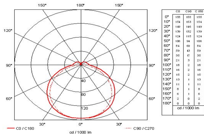
Figure 10-79. Photometry of the luminaire.
