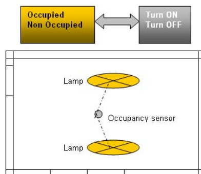
Figure 6-5. Occupancy control scheme.
