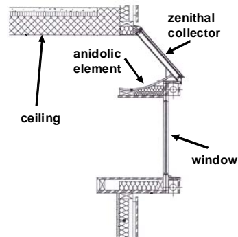
Figure 10-1. Southern facade of the building and a cross section from the facade's system.
