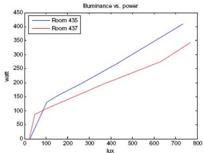
Figure 10-12. Relationship between illuminance and consumed power in the offices.
