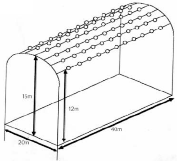
Figure 10-96. Shape of the building.
