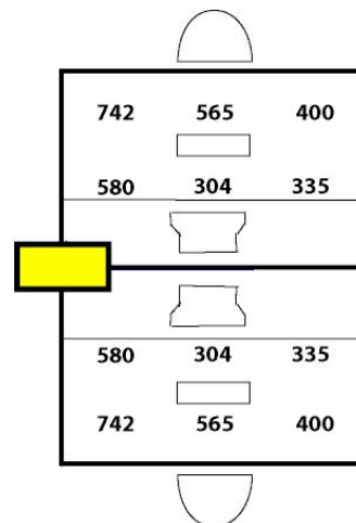
Figure 10-25. Direct-indirect stand-alone luminaire .
