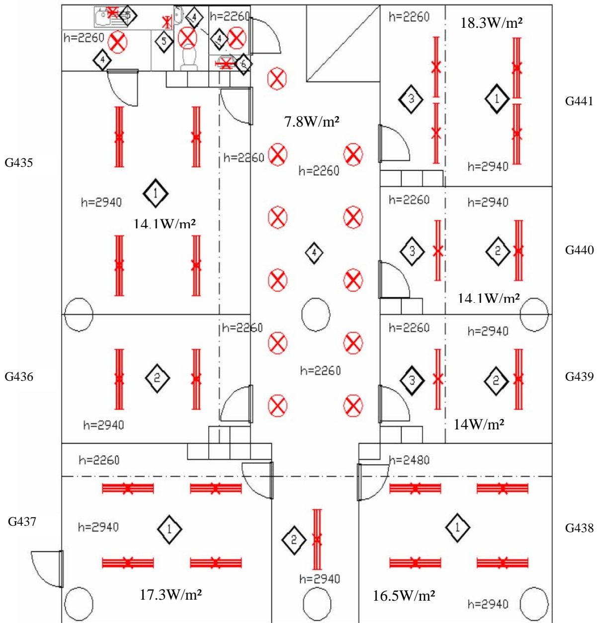
Figure 10-5. Office Plan with the luminaires position.
